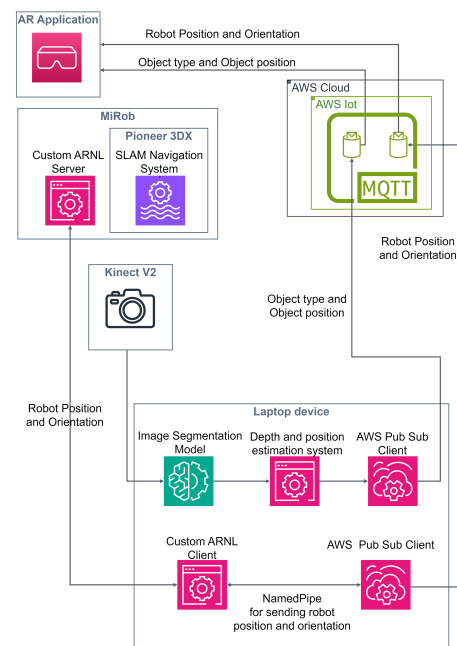
Fig. 1. System Architecture
